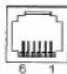
Fig.2-7 Cash Drawer Interface
