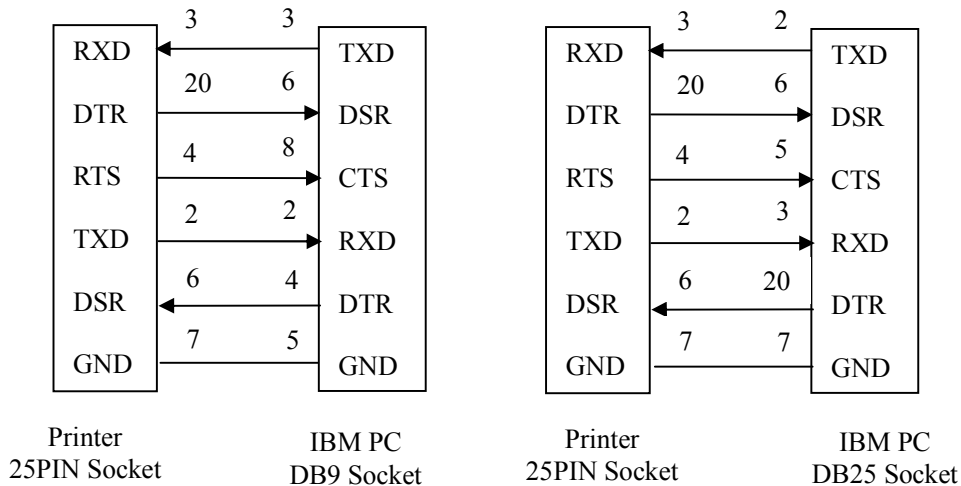
Fig.2-4 Connection between SP-POS88 V and IBM PC Serial Interface Sketch Map
