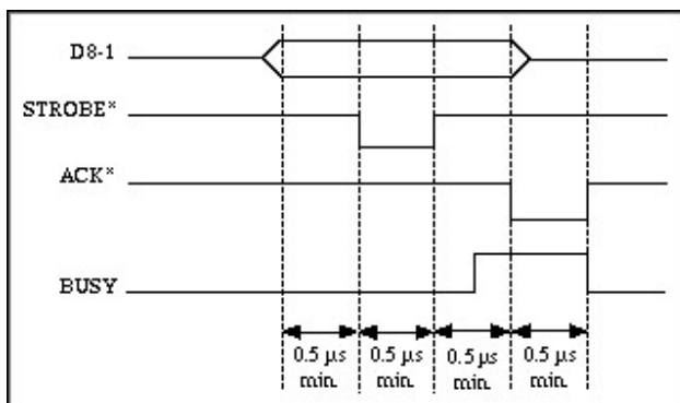
Fig.2-6 Signal Timing Chart of Parallel Interface
